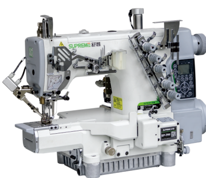
UTC 气动自动上下剪线和抬压脚装置 Pneumatic automatic upper and lower wire cutting and lifting foot device
