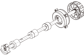
通轴电机 Through-shaft motor
